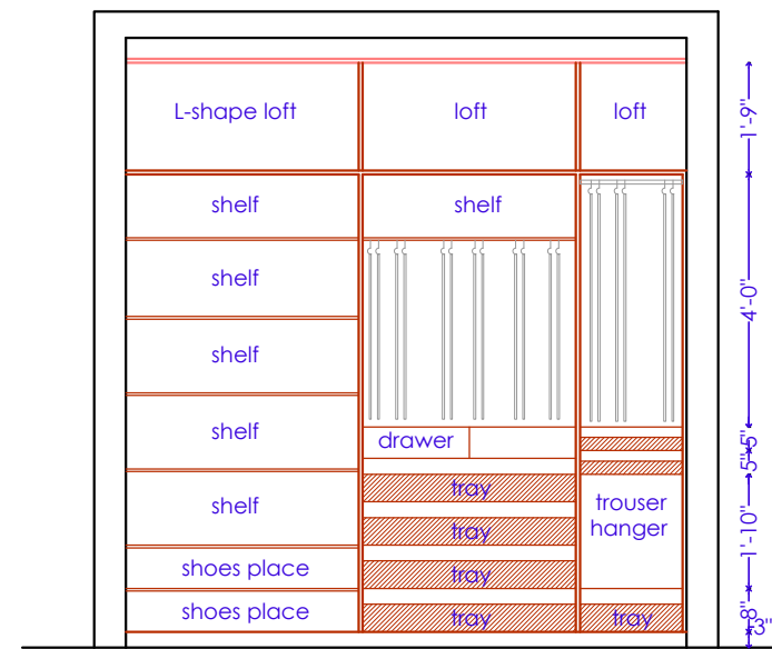
ELEVATION AT 'B
