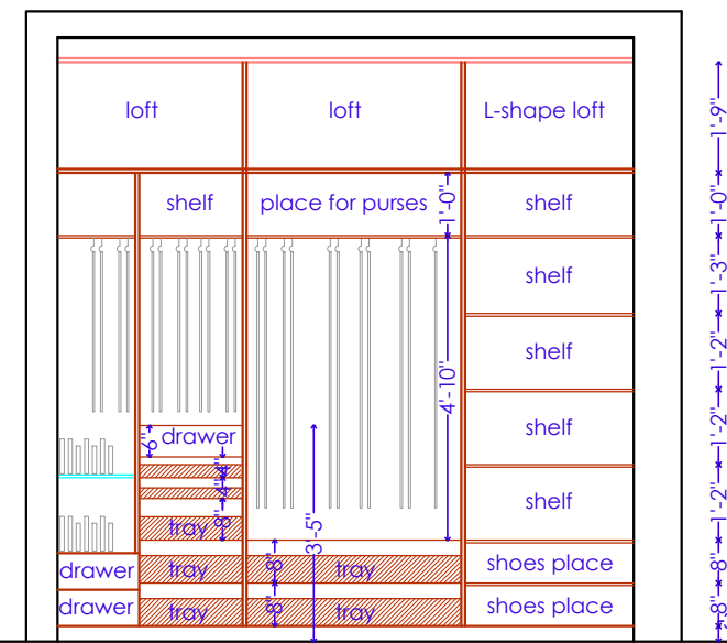
ELEVATION AT 'A
