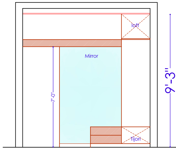
ELEVATION AT 'C
